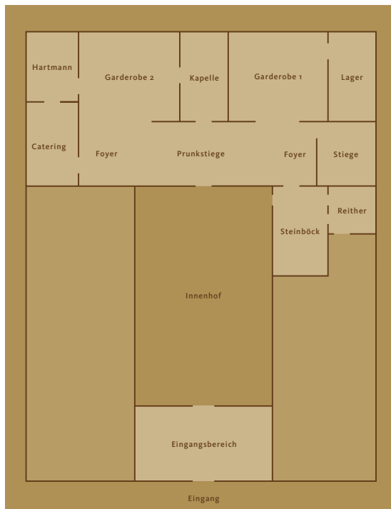
Erdgeschoss/ground floor
